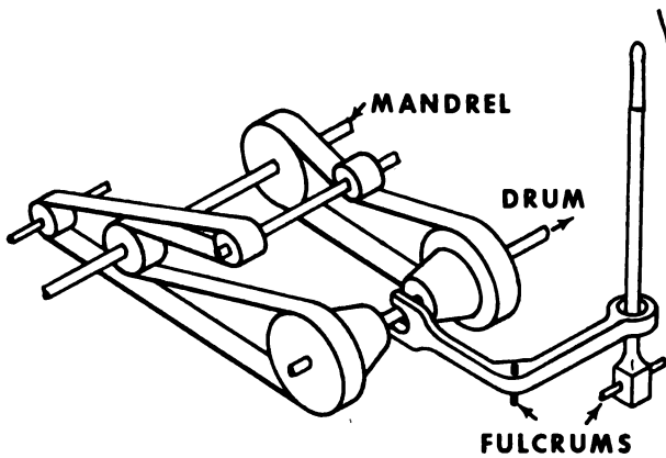
Figure 8-7. Belt-driven feed works with clutch.
